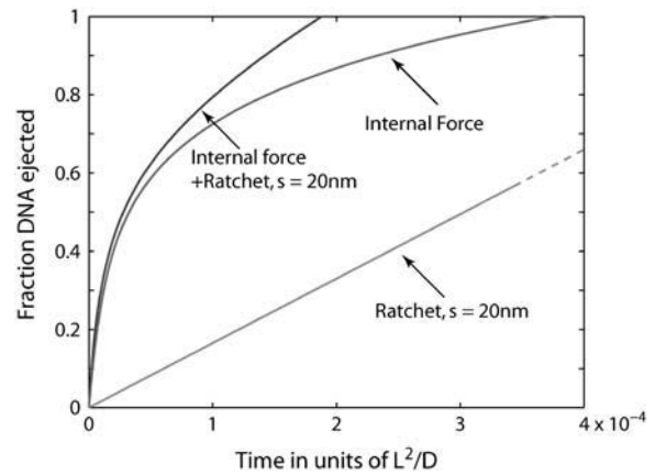
FIGURE 3 The fraction of DNA injected in phage \lambda as a function of time (in units of L^2/D ) in the presence of binding particles that form a ratchet. The DNA injection purely due to the internal force is used as a benchmark, and the spacing between the binding sites s = 20 nm. It can be seen that the ratchet reduces the translocation time. The time required to internalize the genome solely by the ratcheting mechanism (see lower, straight line) is approximately twice the time taken for the purely internal force-driven mechanism.
